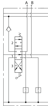
Hydraulic Circuit Hidrolik Devre
